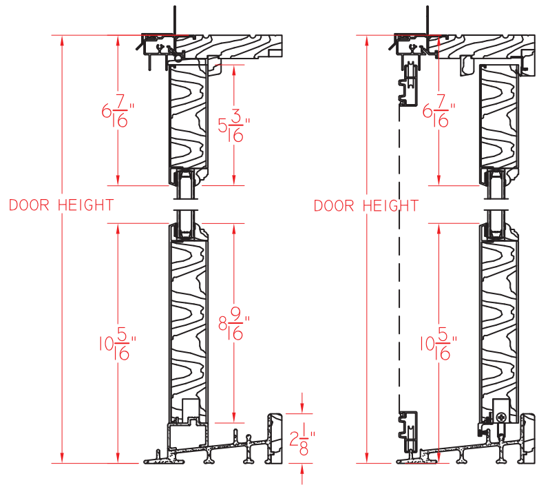
Ⓐ VERTICAL CROSS SECTION
