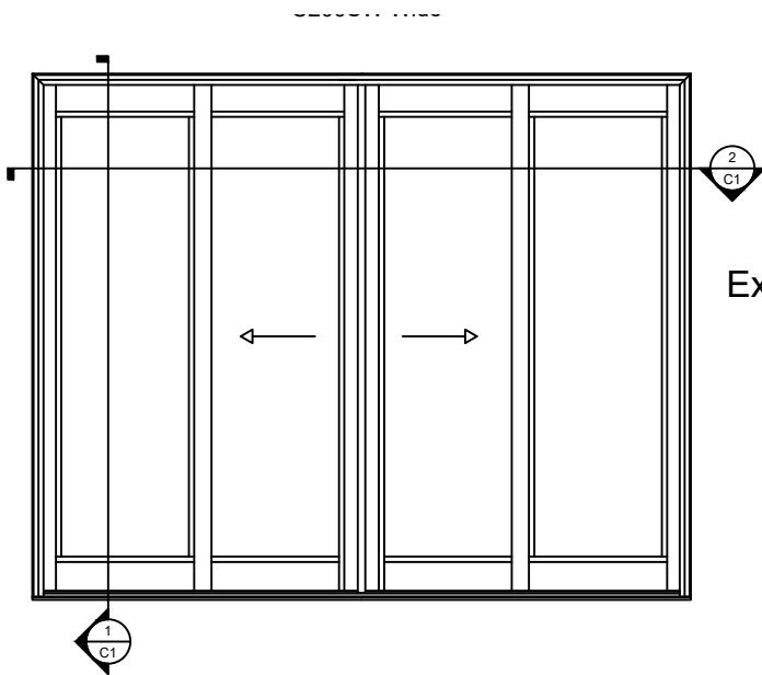
Window Elevation 3/8" = 1' 0"
